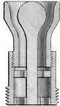
FIG. 3.—Adjustable nozzle.
